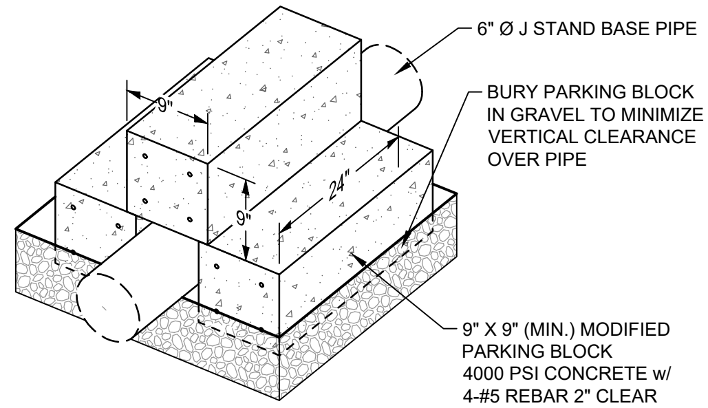
1 J STAND BALLASTING C5 NTS
