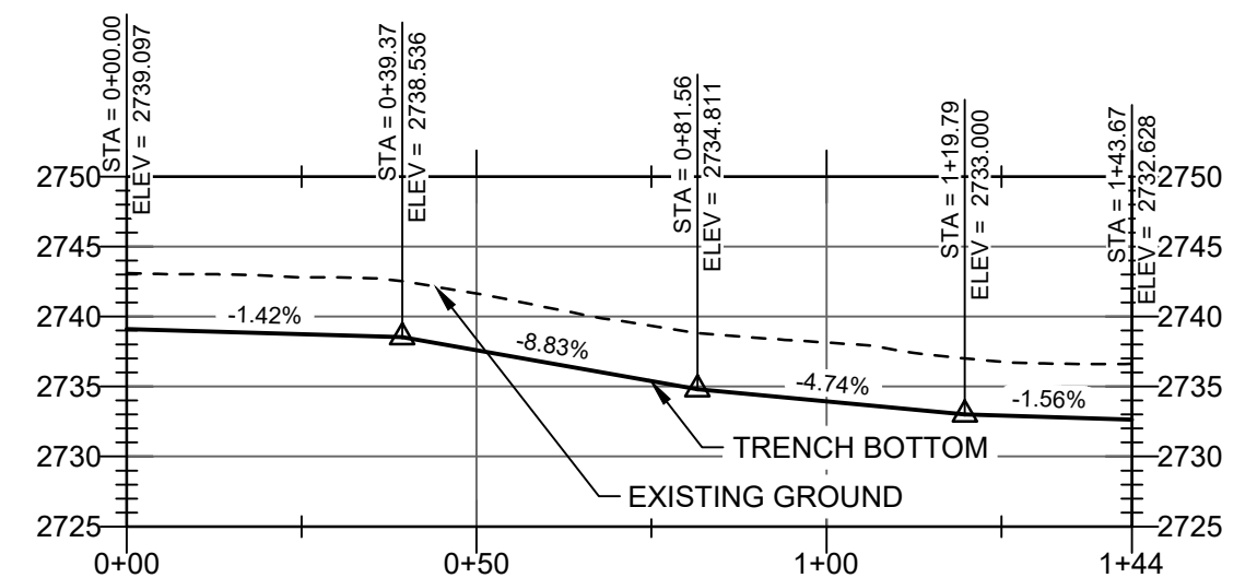
PIPELINE TRENCH CENTERLINE PROFILE
