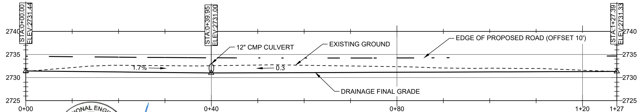
PROPOSED ROAD DRAINAGE CENTERLINE PROFILE SCALE: 1"=10'
