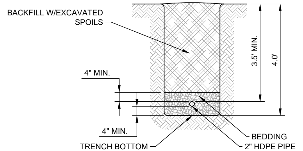
1 4 TYPICAL TRENCH BACKFILL DETAIL SCALE: NTS
