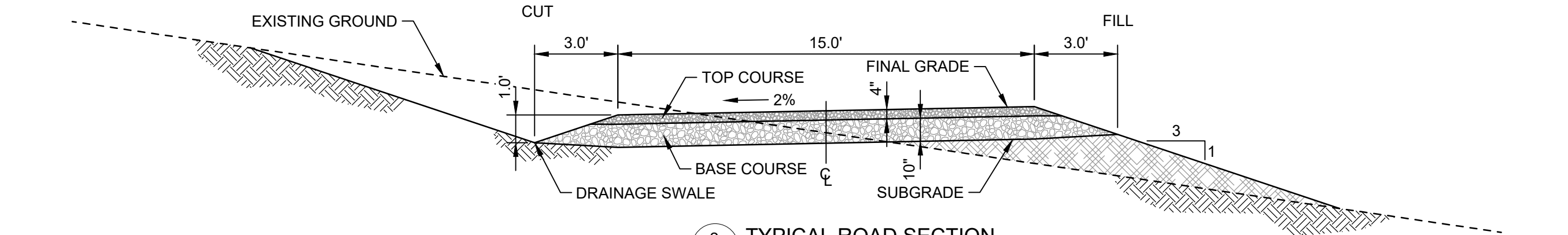
2 C2 TYPICAL ROAD SECTION SCALE: 1"=4'
